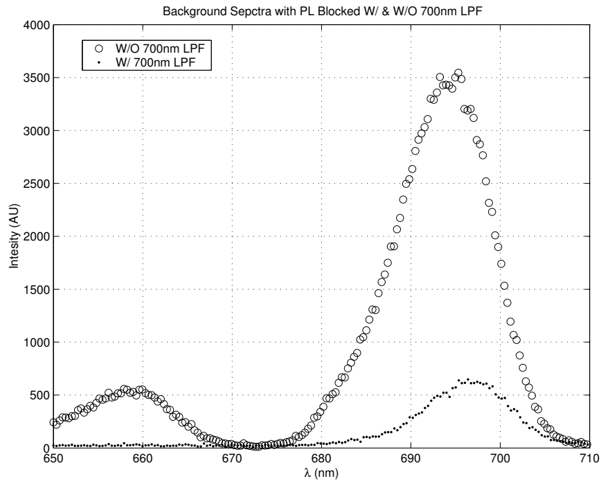
Figure A.1 Background signal level as a function of wavelength with and without a 700nm Long-Pass filter in the crystal pump beam. Above 700nm the signal is cut off by a short pass filter placed in front of the spectrometer.
